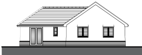
PROPOSED REAR ELEVATION
