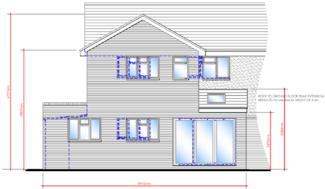
Proposed South Side Elevation
