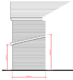
Proposed North Side Elevation
