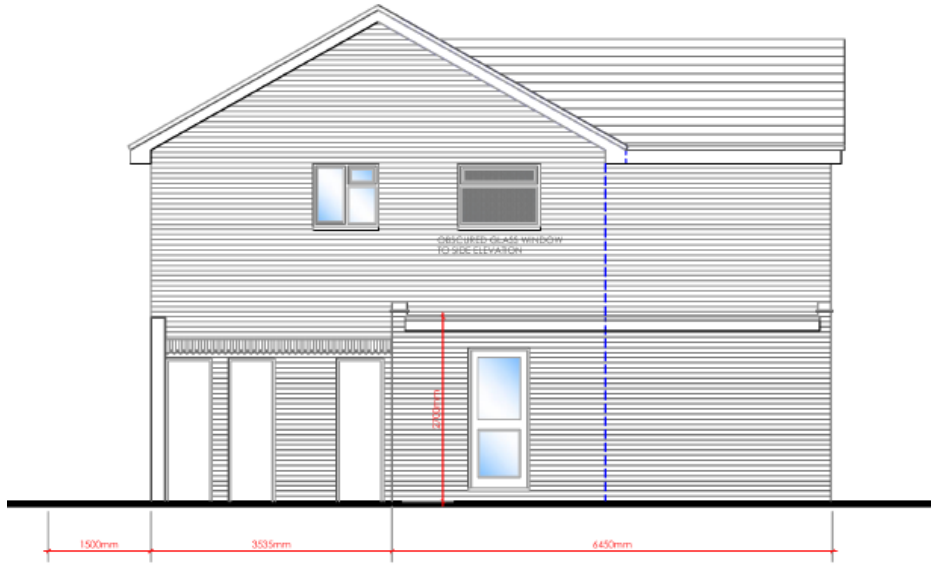
Proposed North Side Elevation
