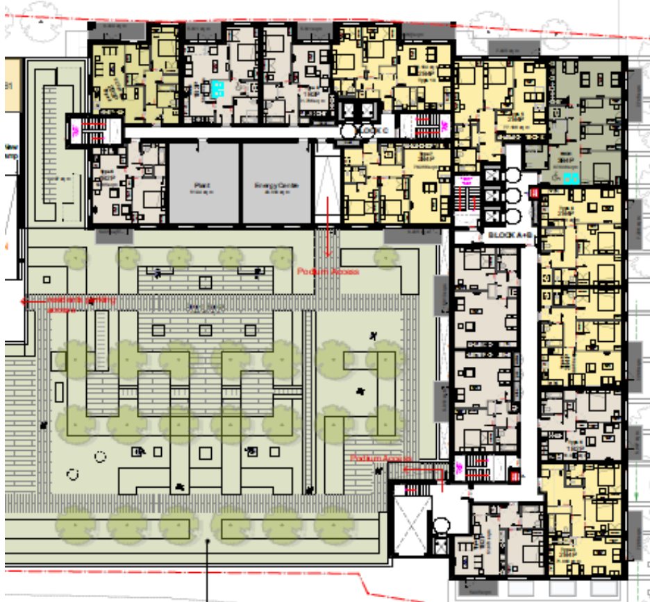
Proposed Floor plan (typical)
