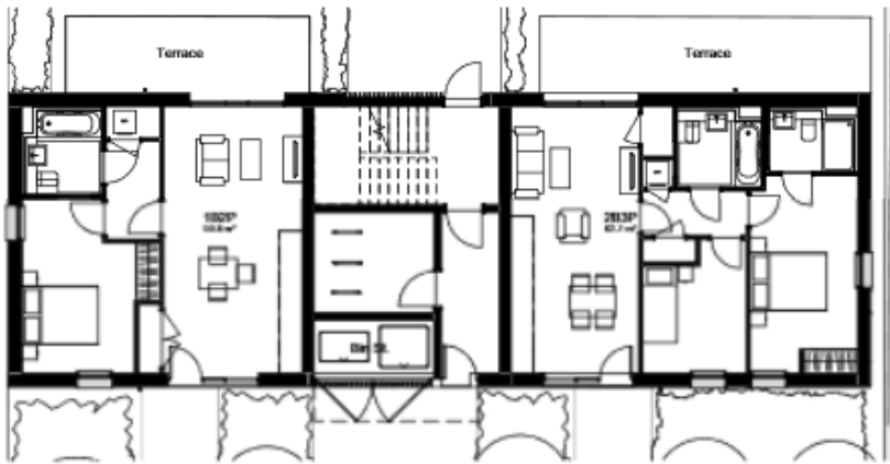
A01D-L00-FFL - Block D 1:100
