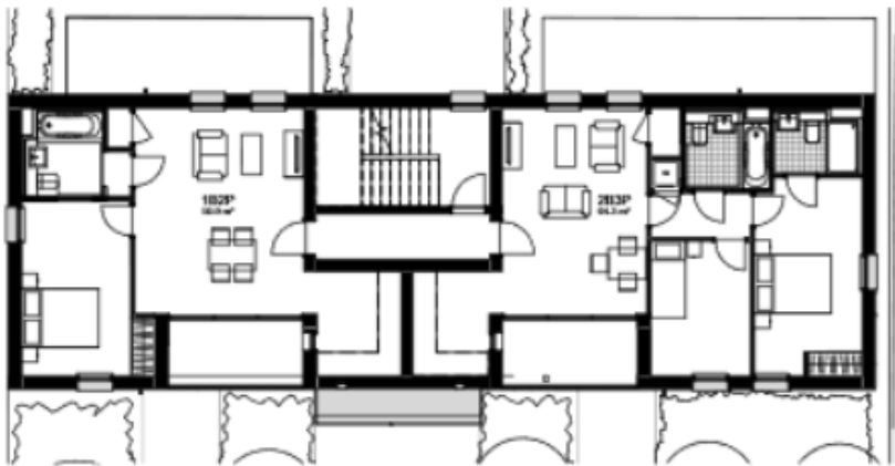
A01D-L01-FFL - Block D 1:100
