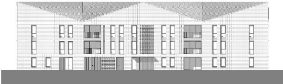
Block C South Elevation 1:100
