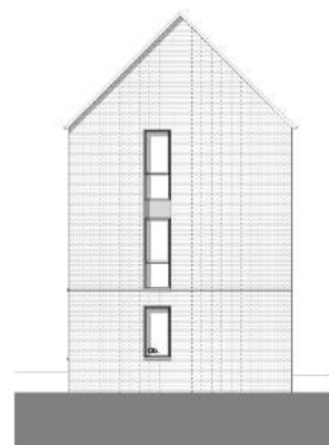
Block D North Elevation 1:100
