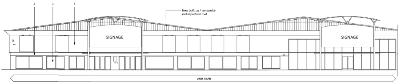
Proposed South East Elevation 1:100
