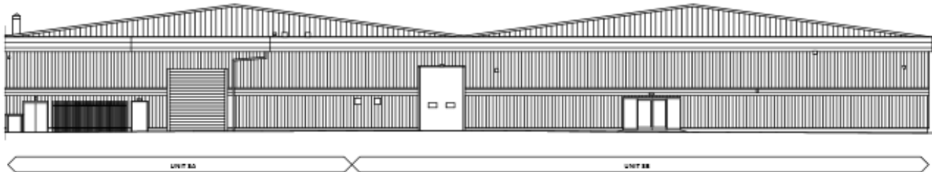
Existing GA Elevation North-West 1:100
