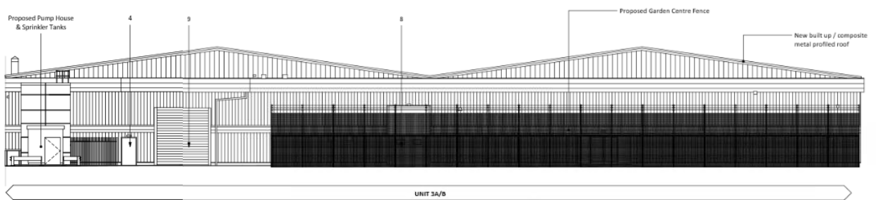
Proposed North West Elevation with Garden Pump House, Sprinkler Tanks & Fence 1:100
