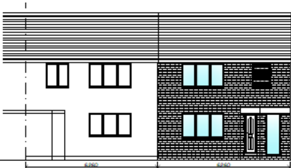
Front Elevation As Proposed
