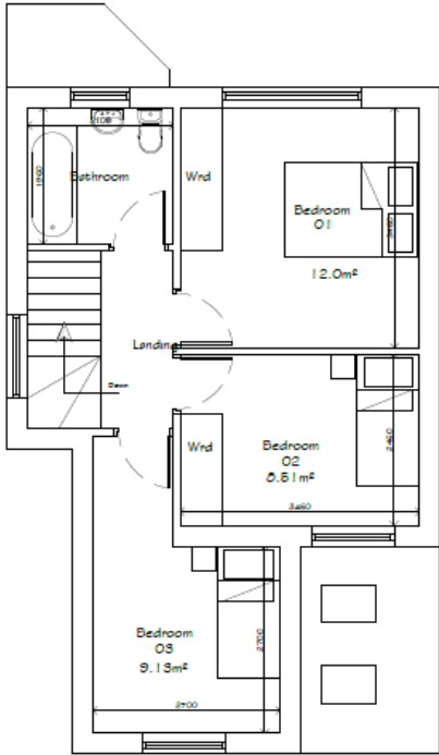
First Floor Plan As Proposed
