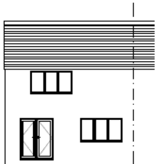
Rear Elevation As Existing
