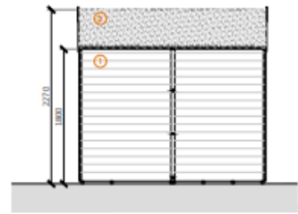
Rear Elevation Scale 1:50
