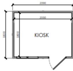
Proposed Floor Plan Scale 1:50
