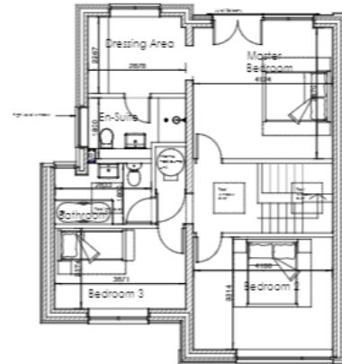
FIRST FLOOR PLAN 68.66m 2
