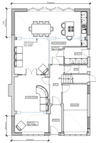
Proposed Ground Floor Layout (Scale = 1:50)
