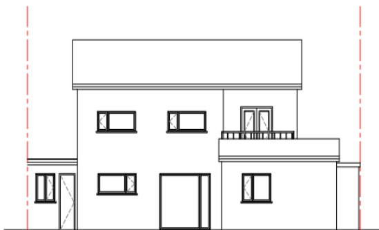
Proposed North Elevation (Rear no change) Scale 1:100
