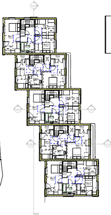
2 01 First Floor Plan 1 : 100
