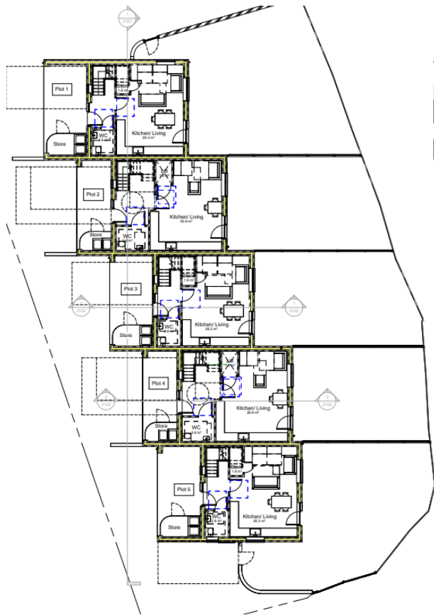
1 00 Ground Floor Plan 1 : 100
