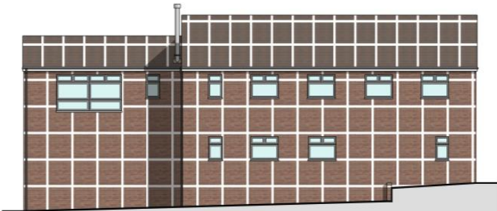
EXISTING WESTERN FACING/SIDE ELEVATION
