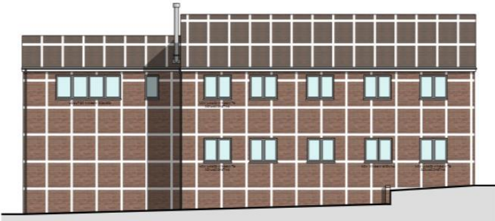
PROPOSED WESTERN FACING/SIDE ELEVATION
