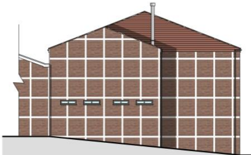
EXISTING NORTHERN FACING /REAR ELEVATION
