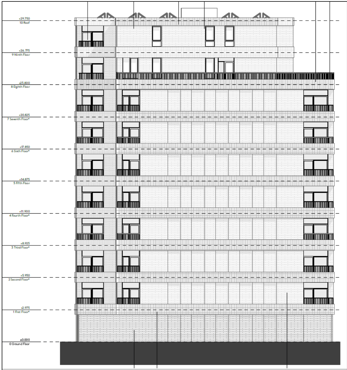
Figure 9 - Proposed North Elevation
