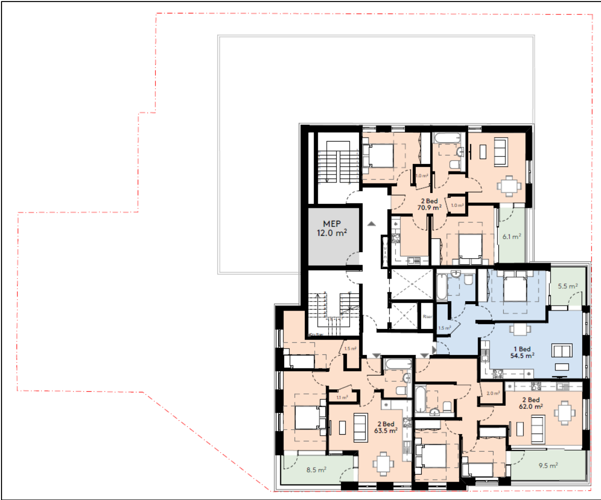
Figure 5 - Proposed 9th Floor Plan
