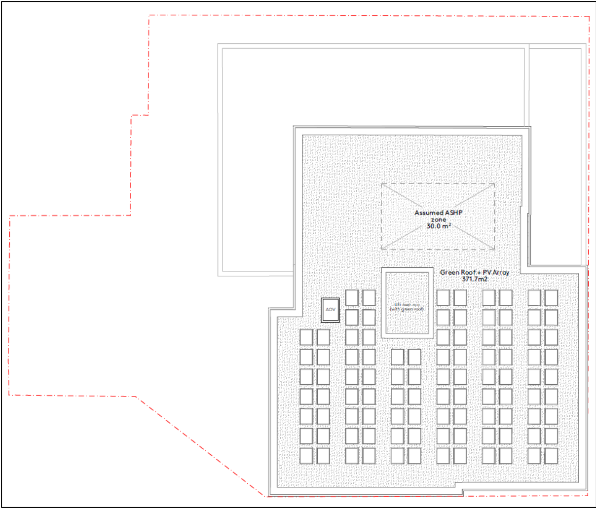
Figure 6 - Proposed Roof Plan
