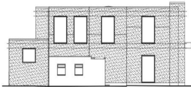
PROPOSED SIDE (1)
