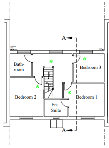
PROPOSED FIRST FLOOR LAYOUT
