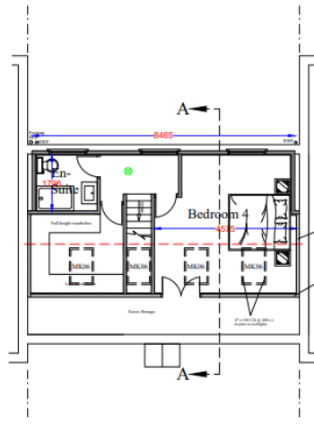
PROPOSED LOFT FLOOR LAYOUT
