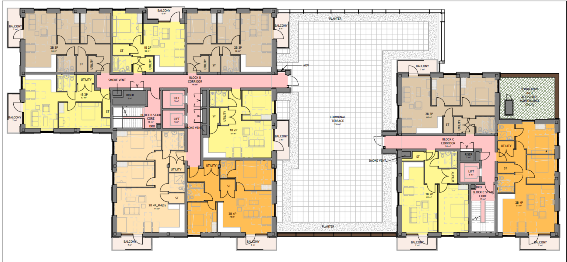
Figure 3 - Block ABC 1st Floor Plan
