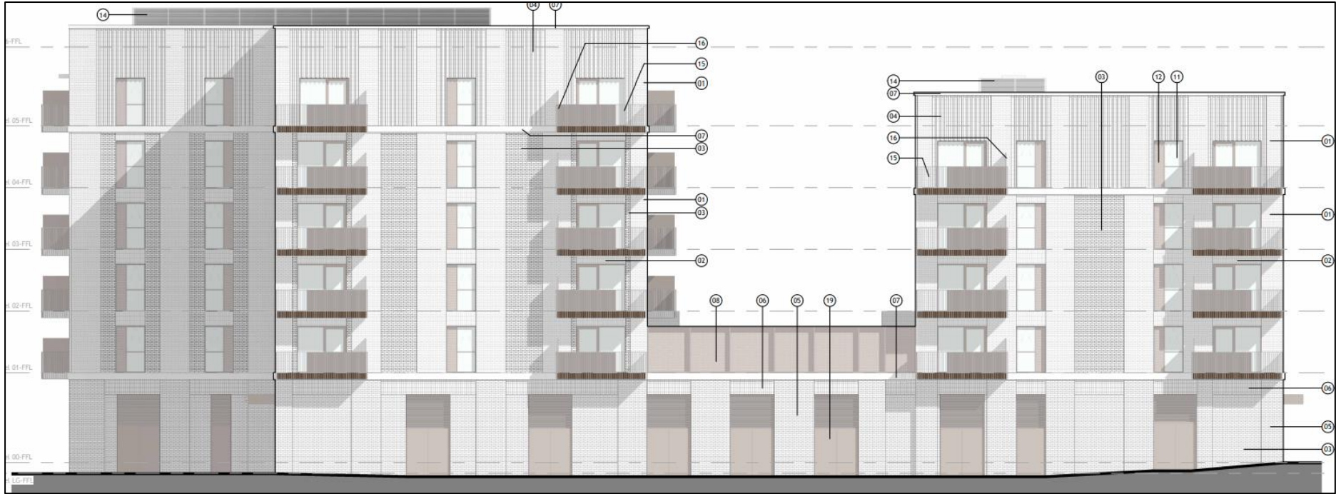
Figure 7 - Block ABC South Elevation
