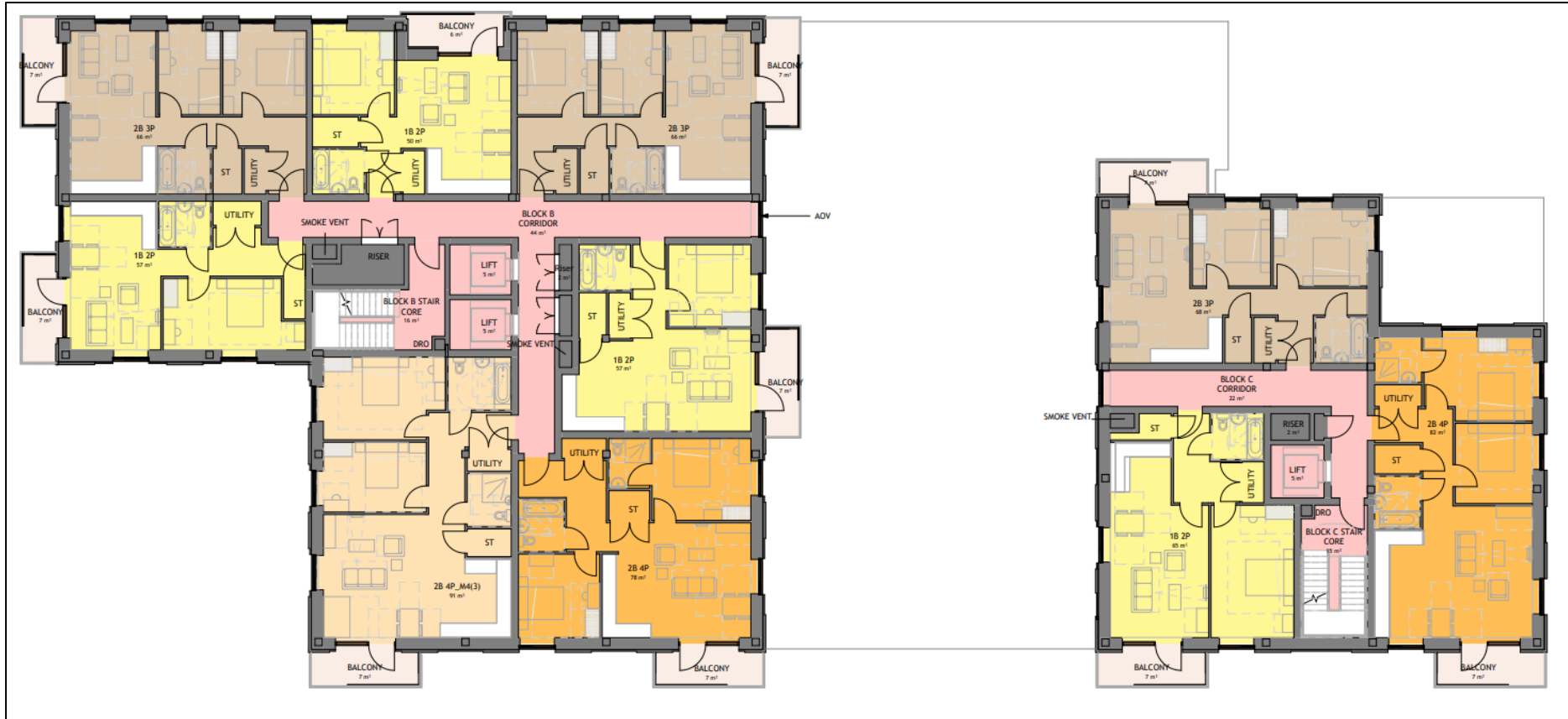
Figure 4 - Block ABC 2nd-4th Floor Plan
