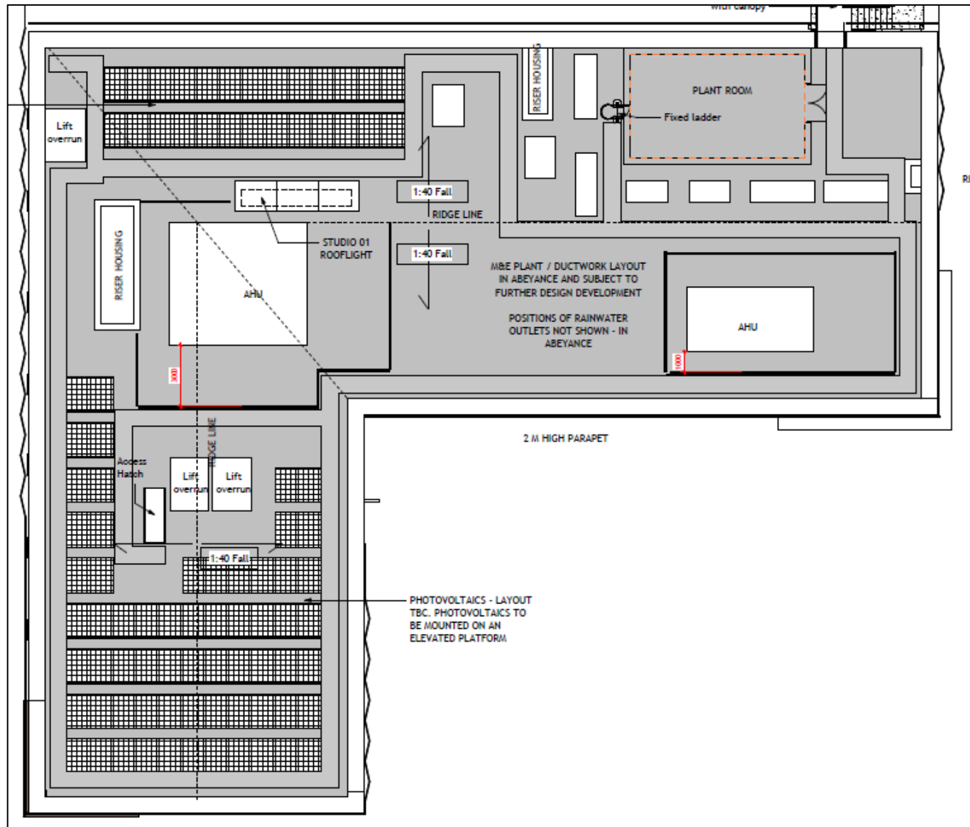
Figure 12 - Block E Roof Plan
