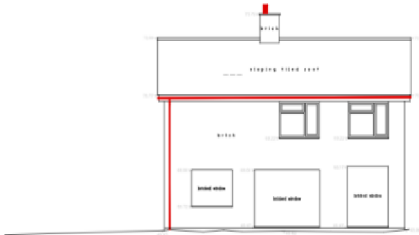
EAST ELEVATION
