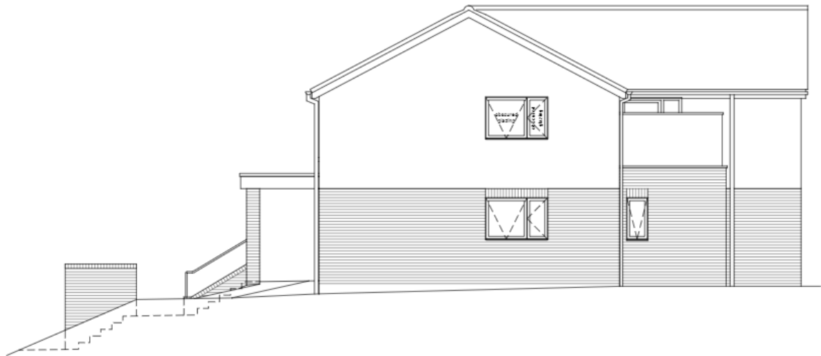
SOUTH ELEVATION
