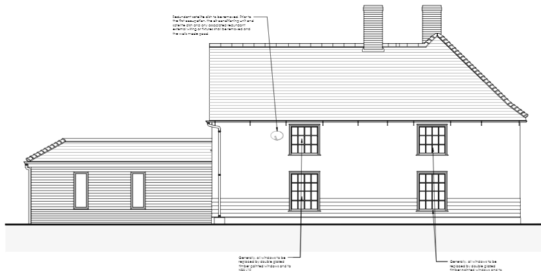
Proposed South-East Elevation (Side Elevation) Scale 1:50
