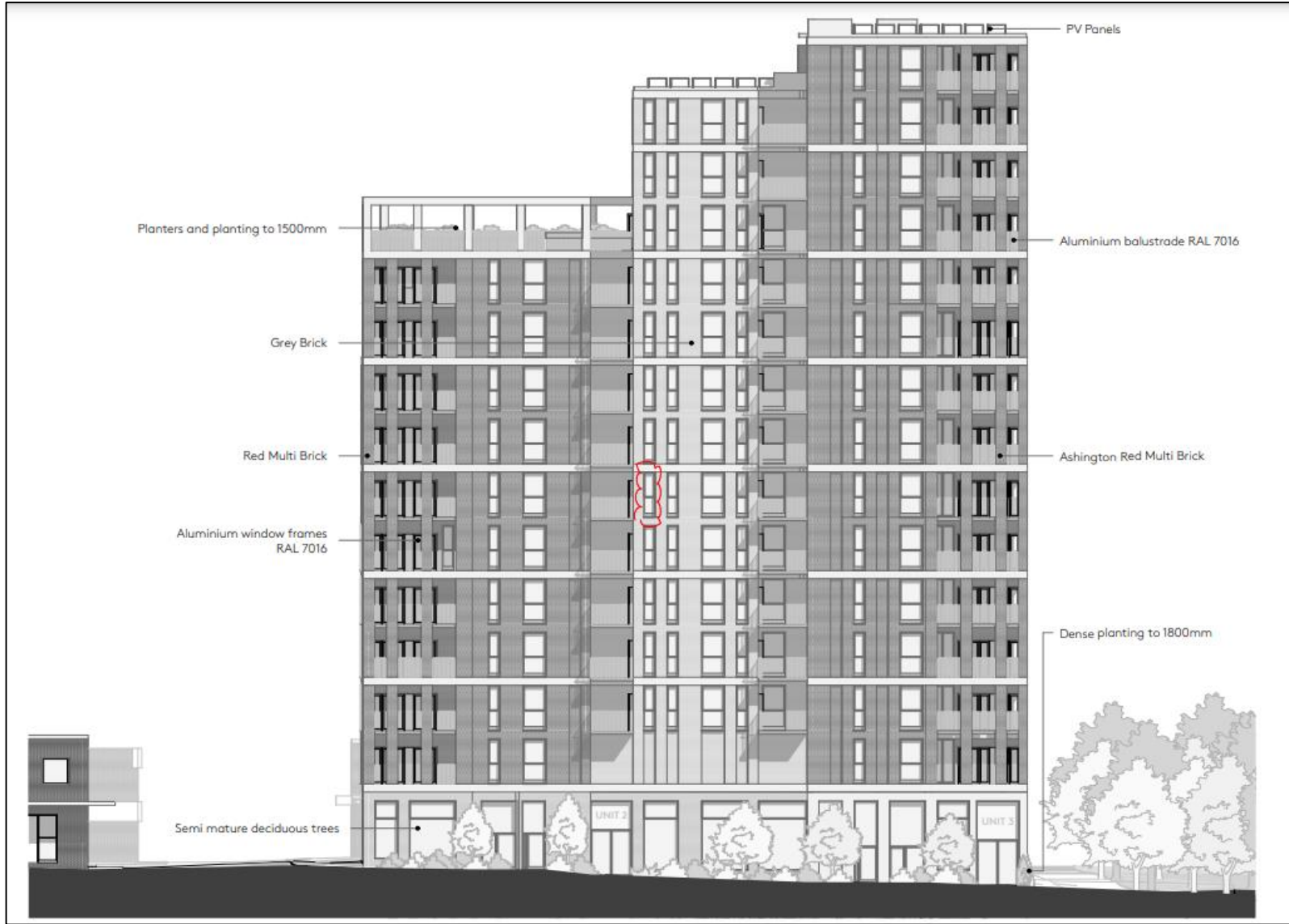
Figure 12: Proposed East Elevation
