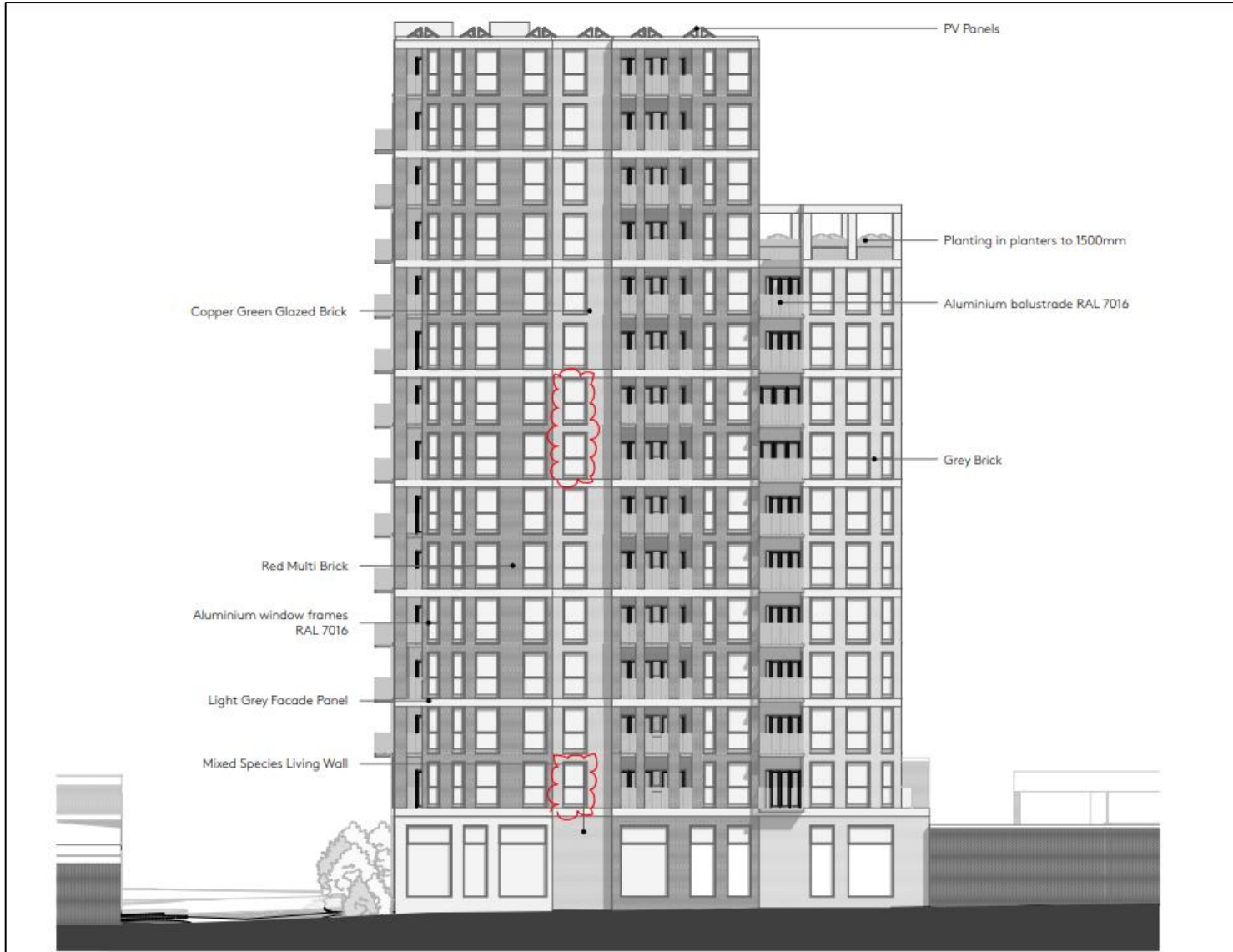
Figure 11: Proposed North Elevation
