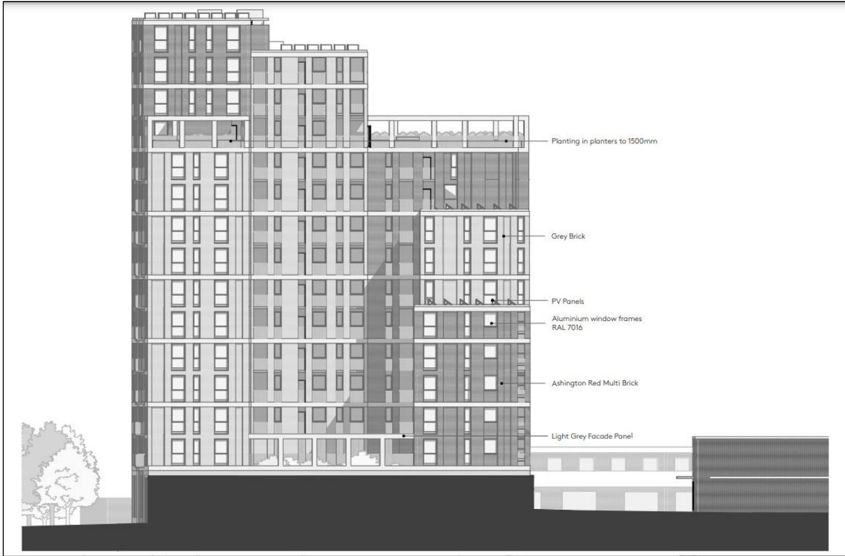
Figure 10: Proposed West Elevation
