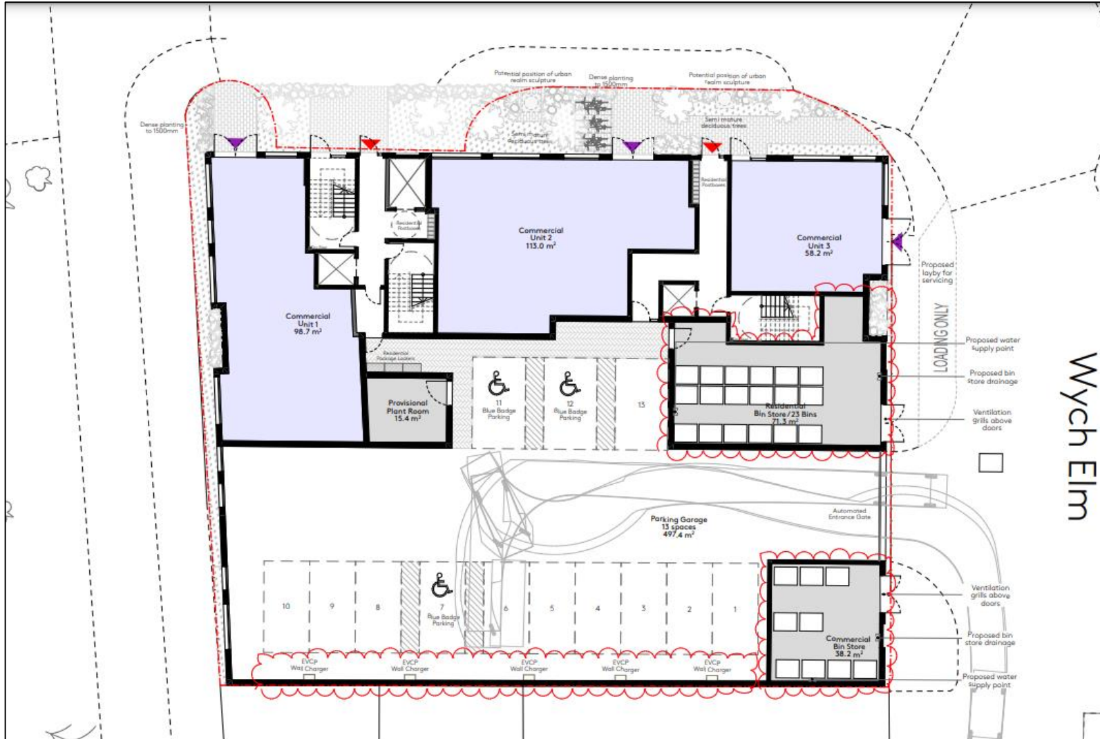
Figure 1: Ground Floor Plan
