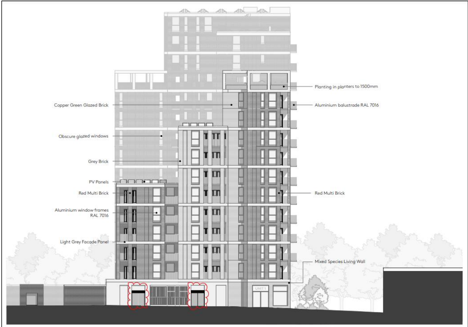
Figure 13: Proposed North Elevation
