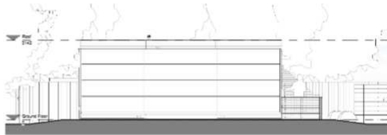
Side Elevation (South) 1 : 50
