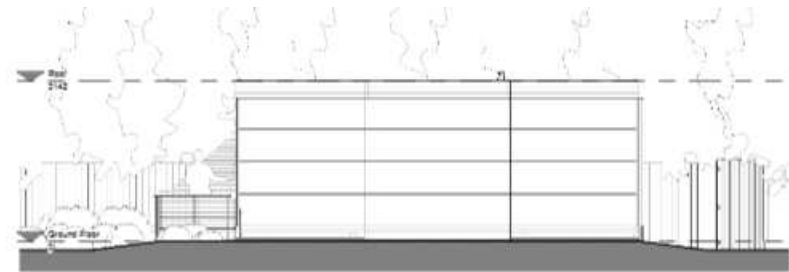
Side Elevation (North) 1 : 50
