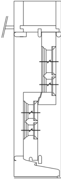
SASH WINDOW SECTION WINDOW TYPE 1
