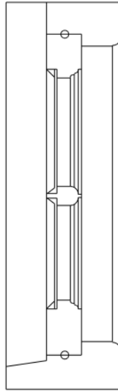
CASEMENT WINDOW SECTION WINDOW TYPE 2
