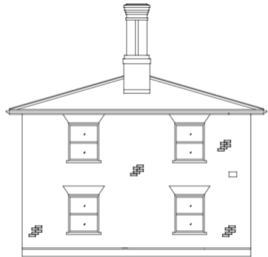
SOUTH ELEVATION
