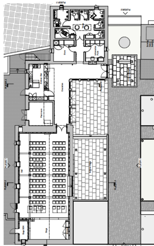
2 Proposed Ground Floor Plan Scale: 1/100
