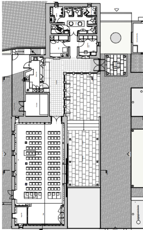
1 Existing Ground Floor Plan Scale: 1/100
