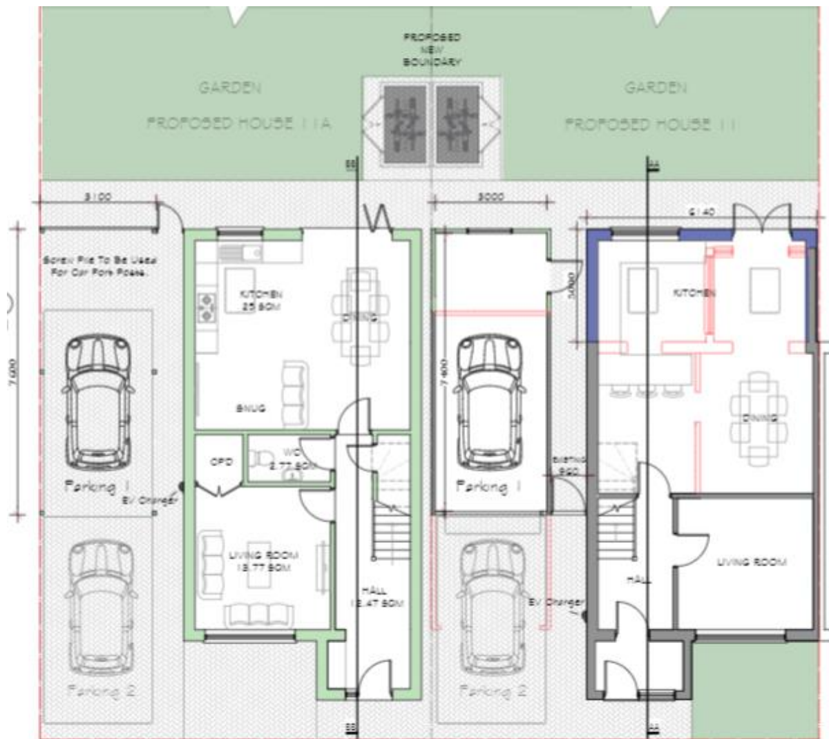
1 PROPOSED GROUND FLOOR PLAN SCALE 1:100
